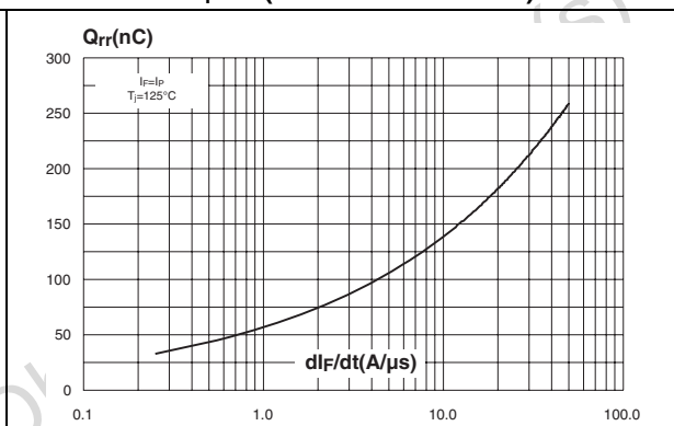
Figure 8. Reverse recovery charges vs. di_F/dt (modulation diode)
